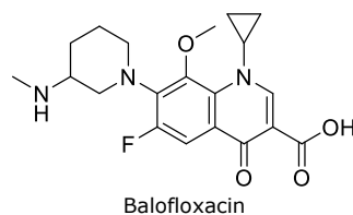
Balofloxacin
