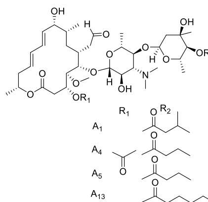
Leucomycin complex
