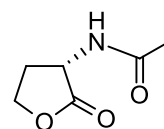
Acetyl-L-homoserine lactone
